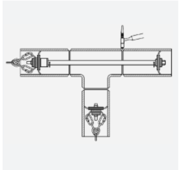
spa root purging system
